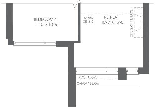
PARTIAL THIRD FLOOR ELEV. B OPTIONAL 4 BEDROOM PLAN
