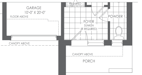
PARTIAL GROUND FLOOR ELEV. B
